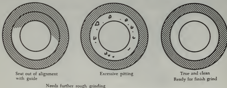
FIGURE 10-9. Valve seat grinding.
